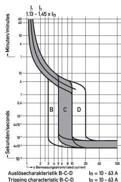
Diagrams miniature circuit-breakers DLS 6i C32-2
