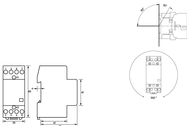
Dimensioned drawing installation contactors HS 2-230AC/25-04
