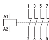
Wiring example installation contactors HS 2-230AC/25-04
