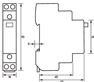
Dimensioned drawing impulse switch (remote switches) RS 230-100
